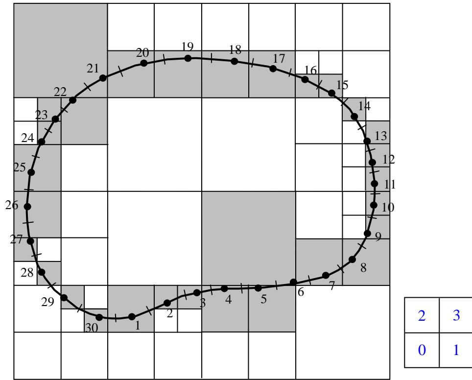
Figure 4. A hierarchical cell structure covering all the boundary elements (the small square on the right-hand side shows the numbering scheme for the child cells of any given cell).
