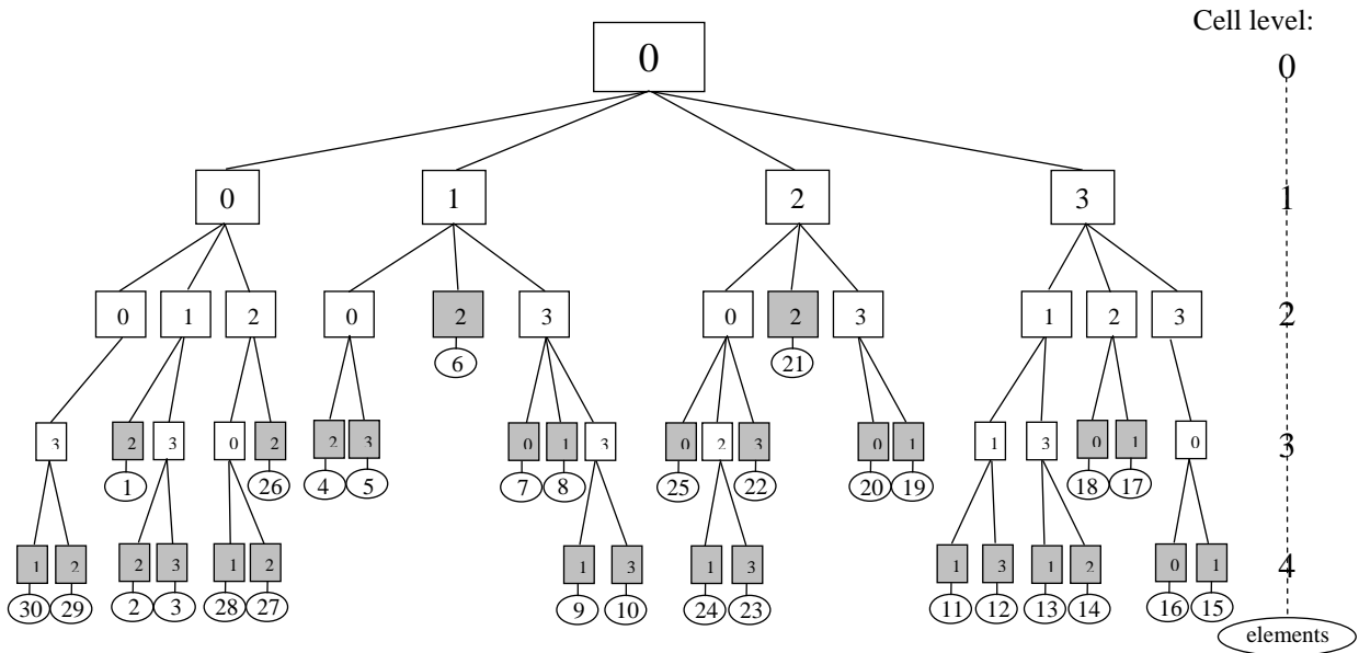
Figure 5. The quad-tree structure.
